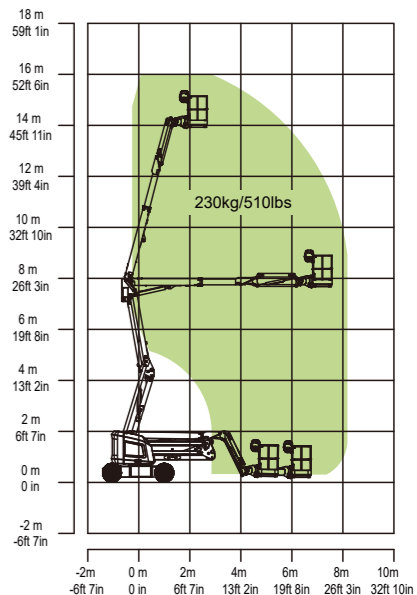
Range of Motion ZA14NJE/ZA14NJE-Li
